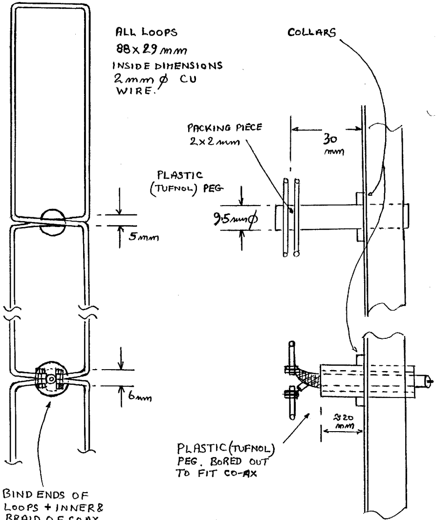
23 CM PANEL ANTENNAS DETAIL OF LOOPS, SUPPORTS AND FEEDER CONNECTION. DRAWING 2.
