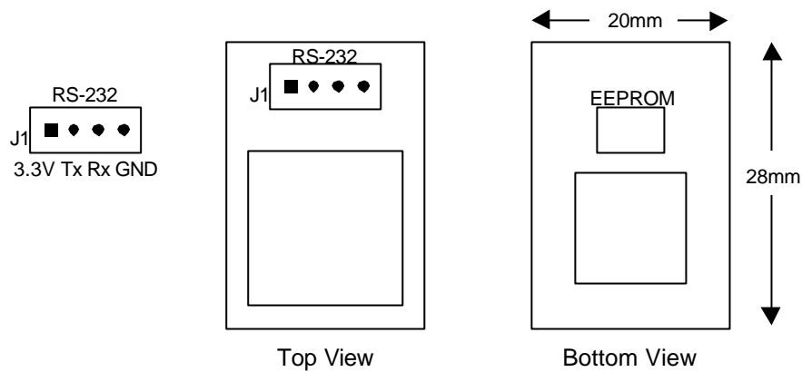
Figure 2 – CJP6380 board layout and serial interface pin
